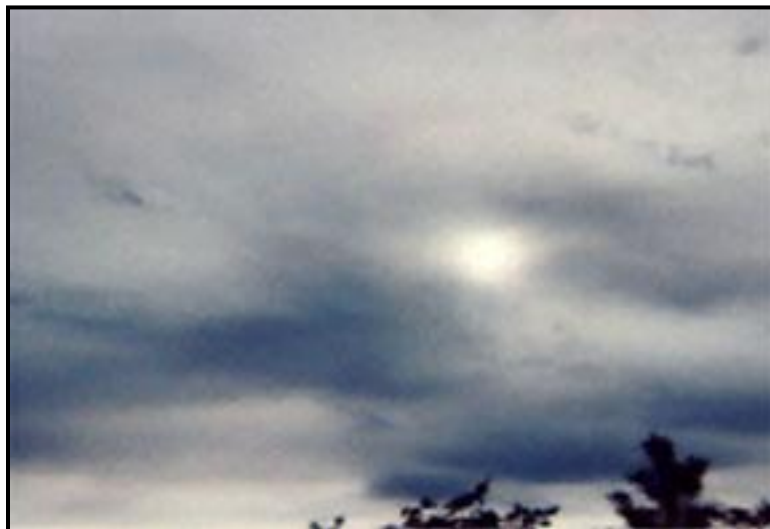
Figure 1-6. Altostratus.
