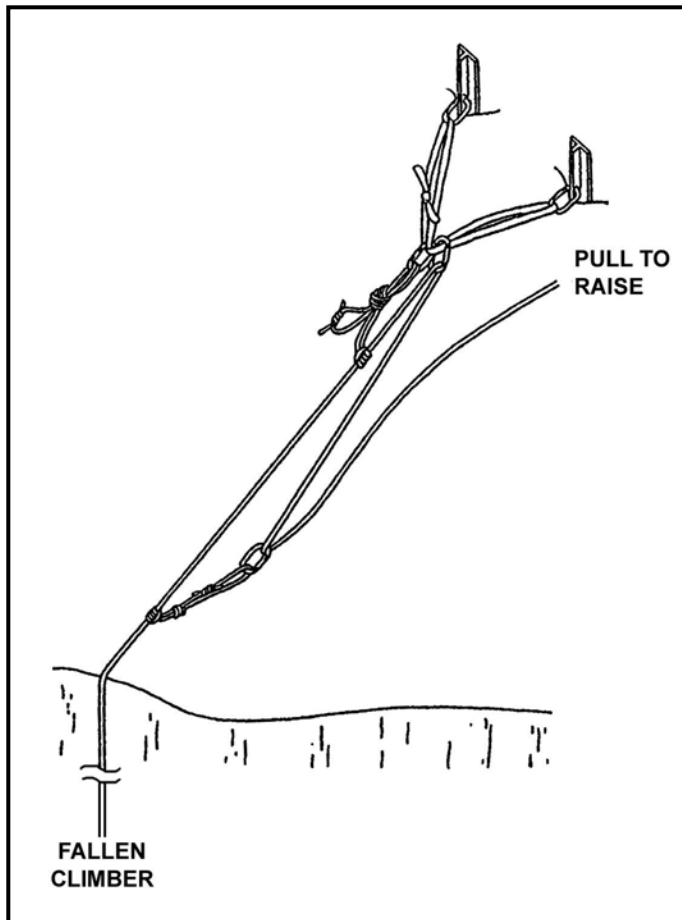
Figure 7-26. Z-pulley system.
